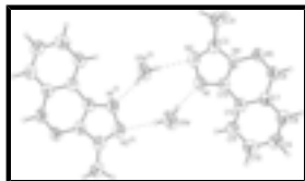
Fig. 1. View of the dimers in the crystal structure of the title compound with labelling and displacement ellipsoids drawn at 50% probability level. Hydrogen atoms are depicted as spheres with arbitrary radii and hydrogen bonding is shown as dashed lines. Symmetry code: (i) -x, 1 - y, -z .
